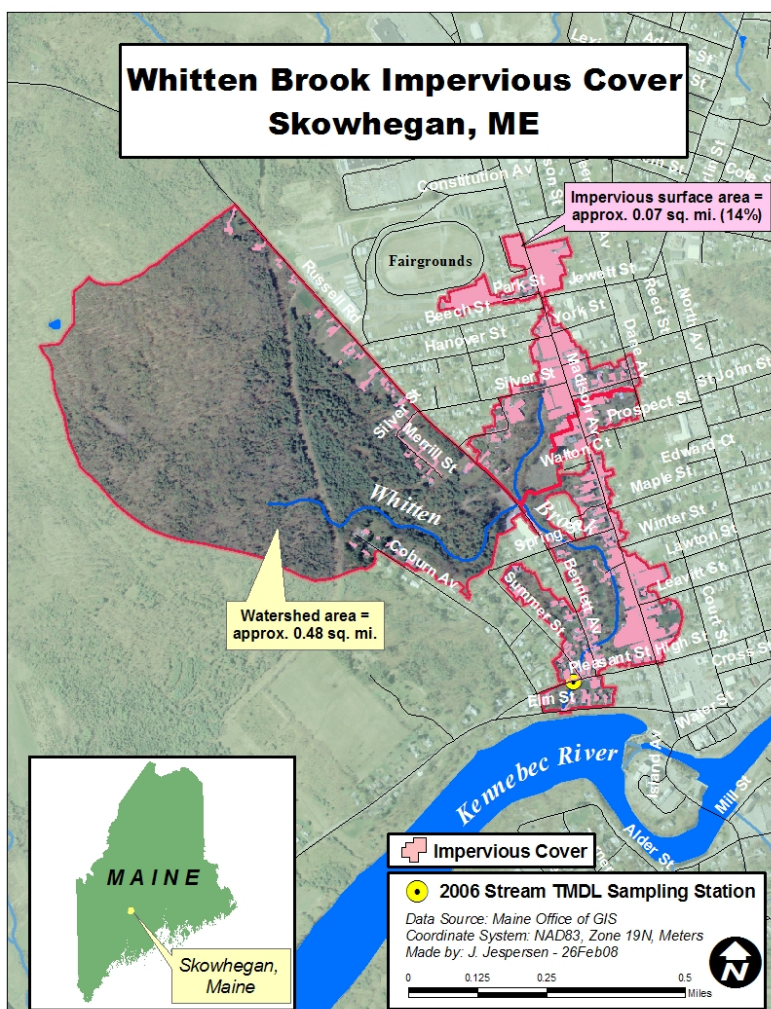
Figure 4. Impervious cover in the Whitten Brook watershed.
