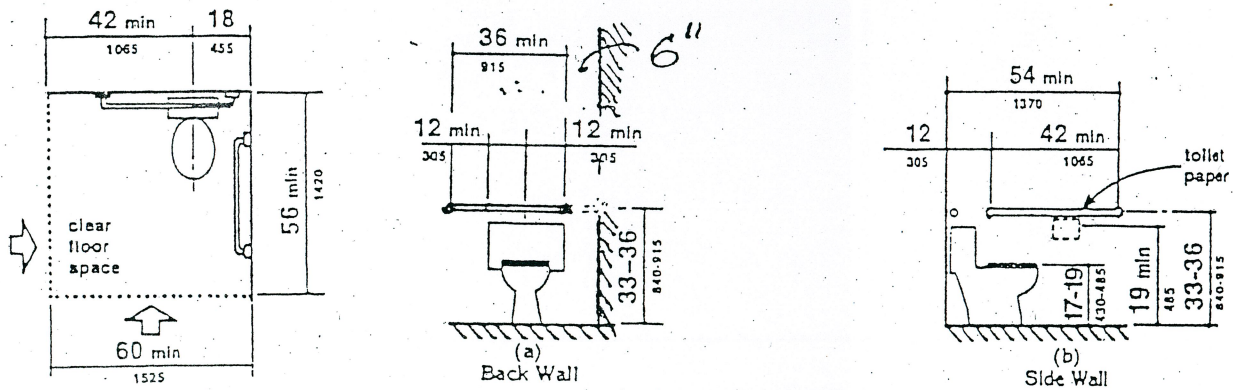
Fig. 29 Grab Bars at Water Closets
